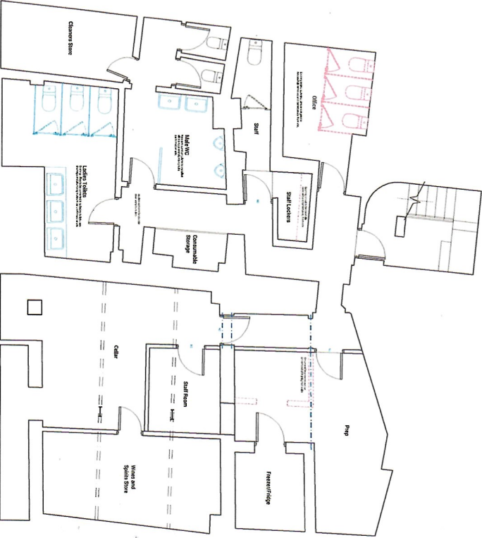
Basement Floor Plan Scale 1:50
